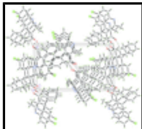
Fig. 2. The crystal packing of the title compound, viewed along the b axis, showing the R_2^2(14) ring motifs. C—H...O intermolecular interactions are shown as dashed lines.
